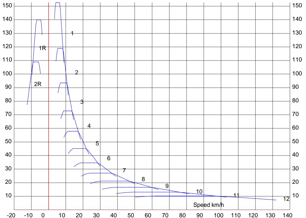
Force F/kN Force Diagram
